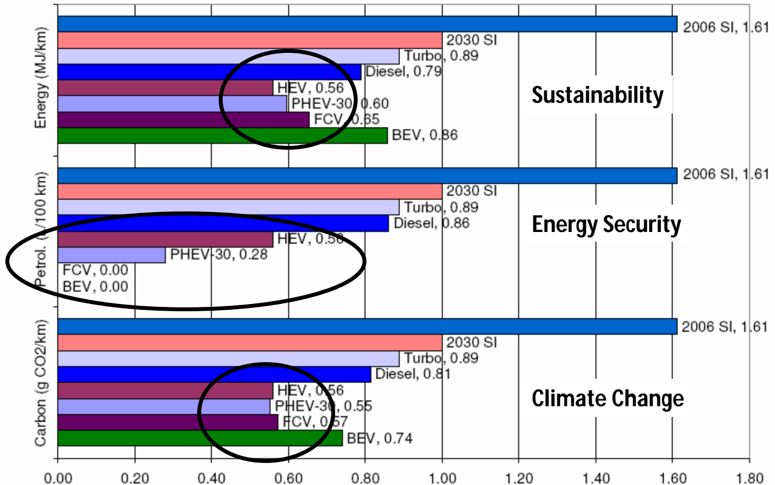
Figure 55: Relative Energy, Petroleum (in Gasoline Equivalent), and GHG Emissions of vehicle options, compared to a 2030 NA-SI
